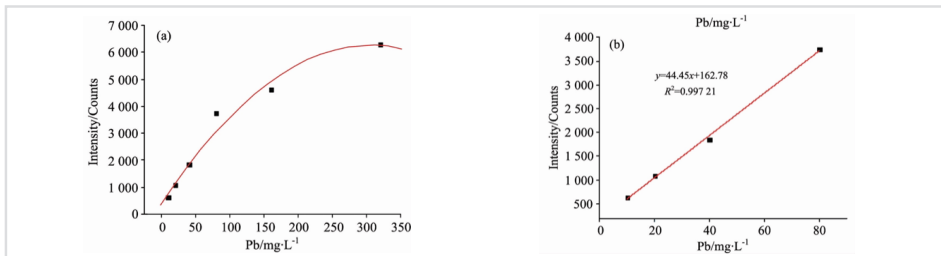
Emission intensity of Pb at different concentration in the solution (a) 10-320 mg/L, self-absorption occurs at higher ion concentrations; (b) 10-80 mg/L
