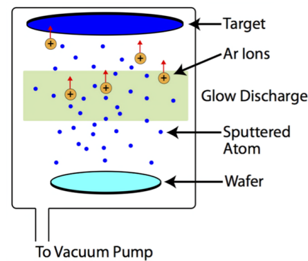
PVD sputtering chamber setup (Ar ions bombard the target, and sputtered atoms are deposited onto the wafer.)
