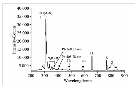
Emission spectrum of \text{Pb}(\text{NO}_3)_2
