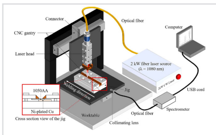
Schematic of experiment setup for laser dissimilar welding and OES.
