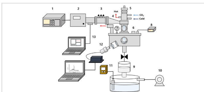
Experimental Setup: The system includes a microwave plasma generator, a plasma-liquid reactor for lithium recovery, a plasma detection system, and a collection device for Li 2 CO 3 products.
