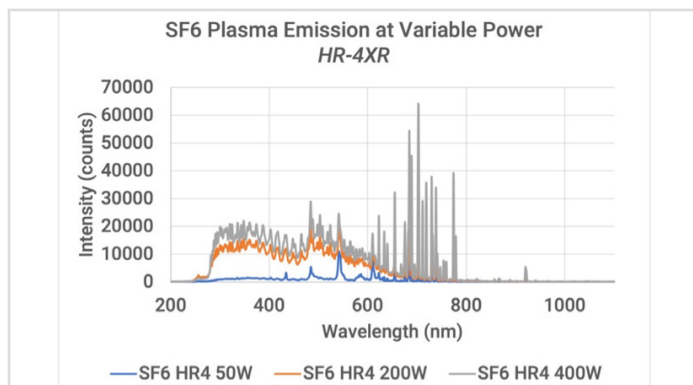
\text{SF}_6 Plasma Emission at Variable Power
