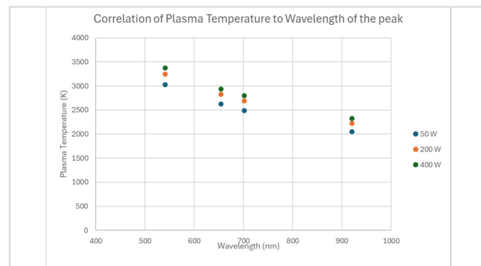
Correlation of Plasma Temperature to Peak Wavelength
